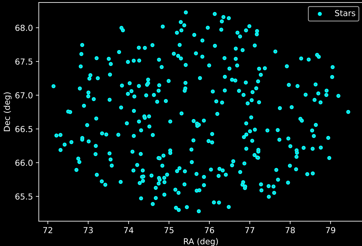
APOGEE DR17 Field: [109+08] Proper Motion Vectors for Gaia Star Field (n= 278)
