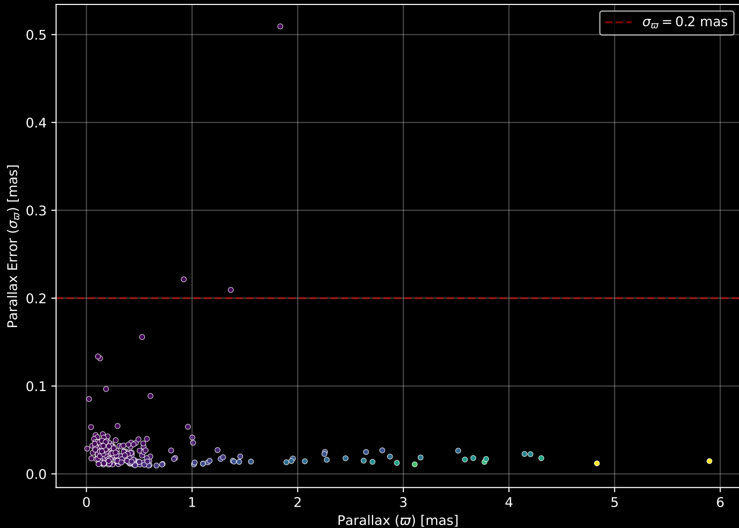
APOGEE DR17 Field: [109+08] Parallax Quality (n= 278)
