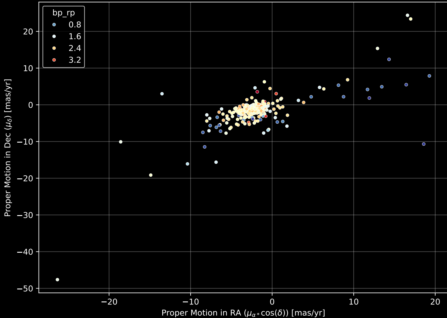
APOGEE DR17 Field: [109+08] Proper Motion Diagram (n= 278)
