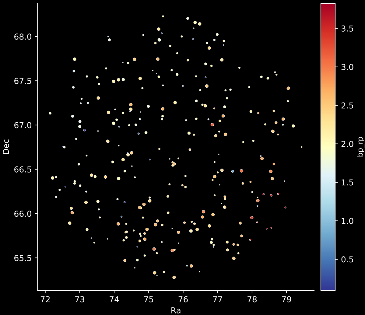
APOGEE DR17 Field: [109+08] Stars: 278
