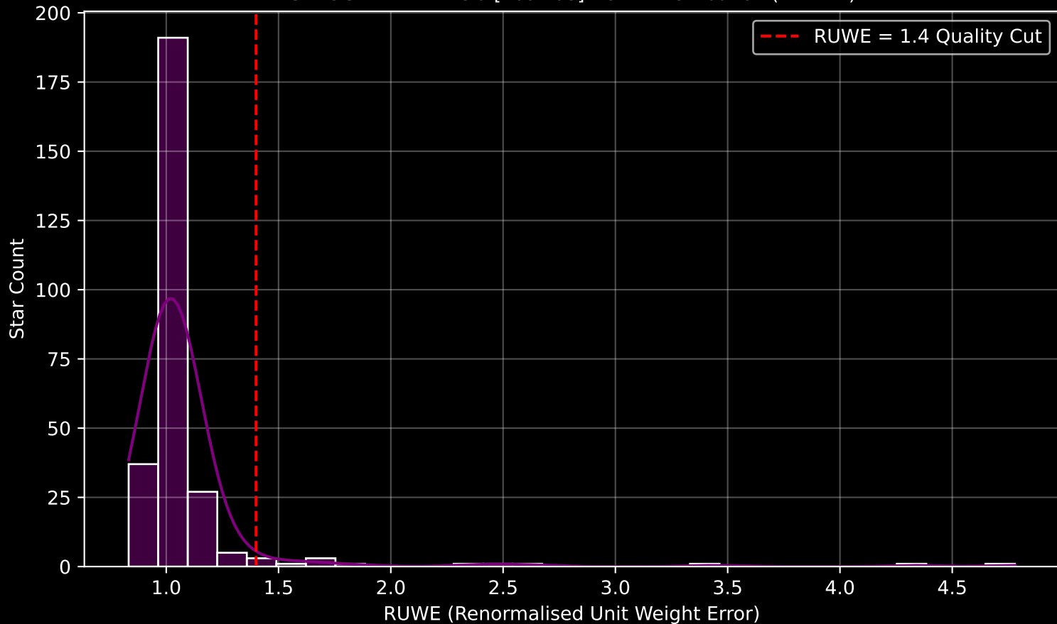
GAPOGEE DR17 Field [109+08] RUWE Distribution (n= 274)
