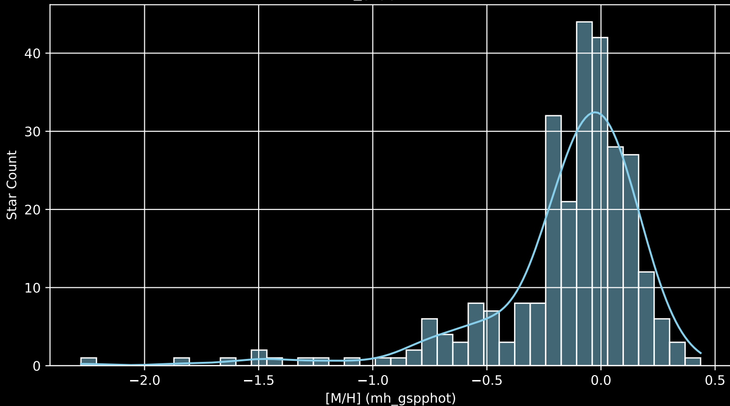
APOGEE DR17 Field: [109+08 [M/H] (mh_gspphot) (n= 276)
